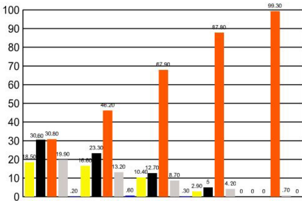
Question 20 : % answers correct by band range
